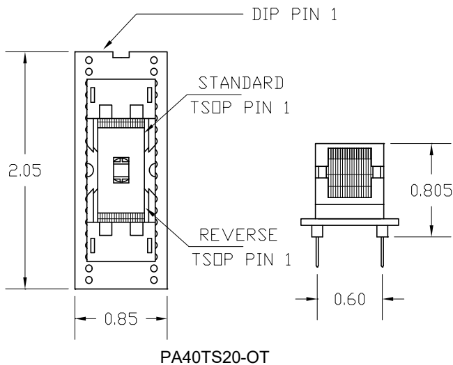
PA40TS20-OT
